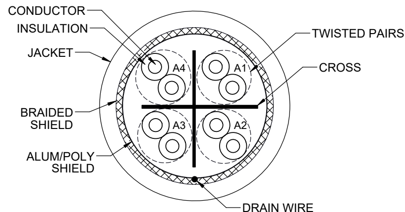
CROSS-SECTIONAL VIEW
