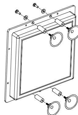
HGX-PMT08 – Window Mounting Kit
